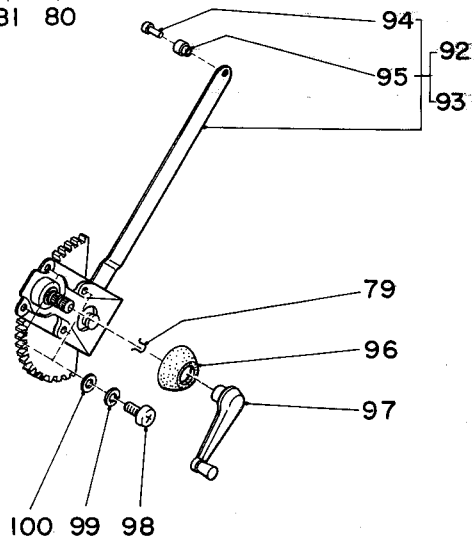
DETAIL "I"
