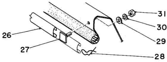
DETAIL "A"
