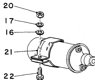
DETAIL "E"
