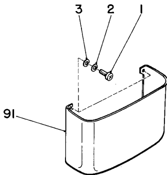
DETAIL "H"
