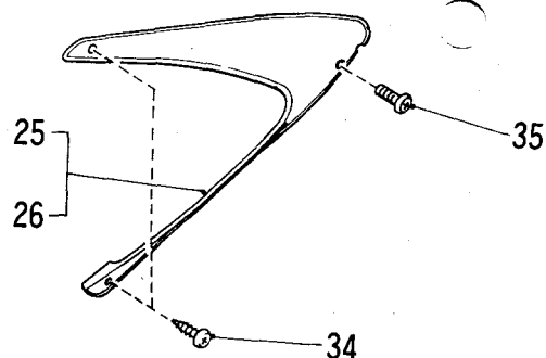
DETAIL "H"
