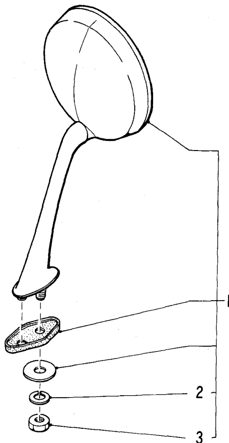
DETAIL "A"
